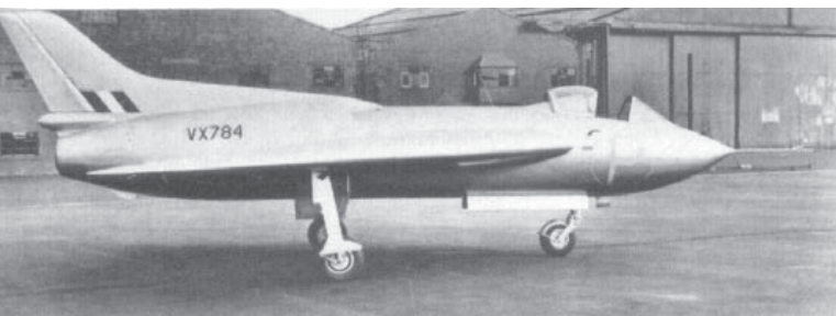
Left: The original Avro 707 prototype, VX784, which crashed on 30th September 1949, less than one month after its first flight, killing the pilot, S. E. Esler. Right: The Avro 707B, VX790, covered by Air Ministry Specification E.15/48, in its original form with a divided air intake for the Rolls-Royce Derwent turbojet. (Photos: Ministry of Supply)
