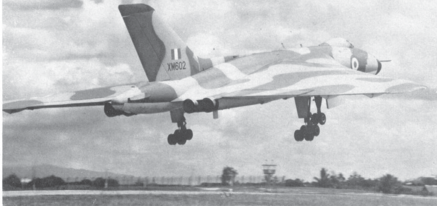
A Vulcan B.2 seen just after unsticking, showing details of the tail cone which contains radar countermeasures equipment.
